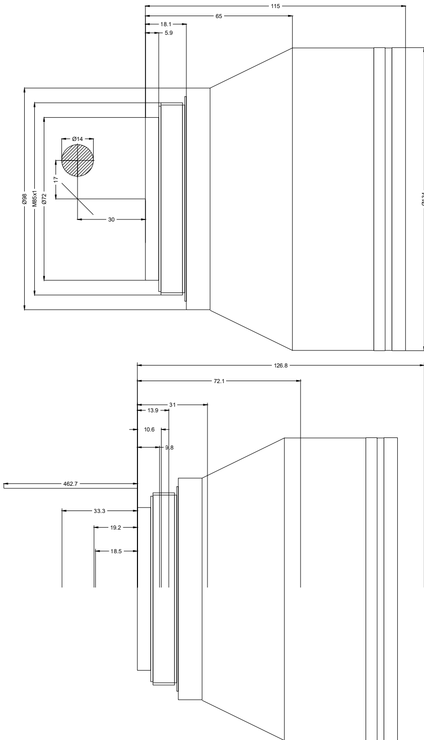
F-Theta lens
