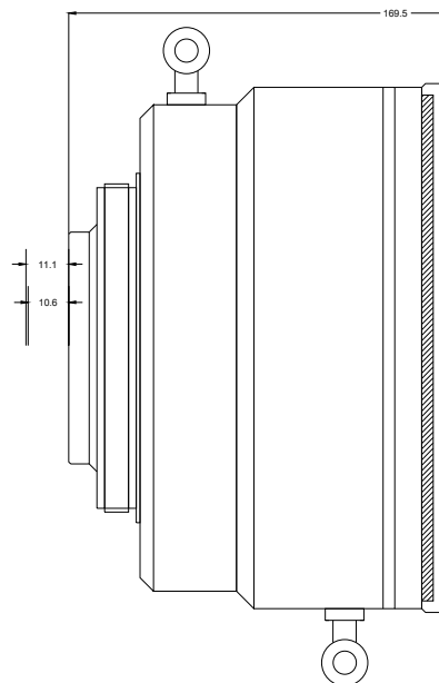
F-Theta lens
